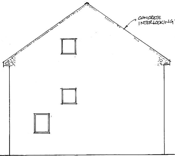
SIDE ELEVATION TO N°1
